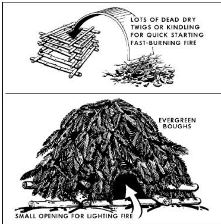
Figure III-5. Smoke Generator
